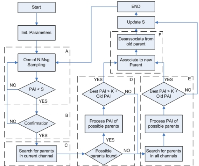
Figure 5. The proactive re-association mechanism
