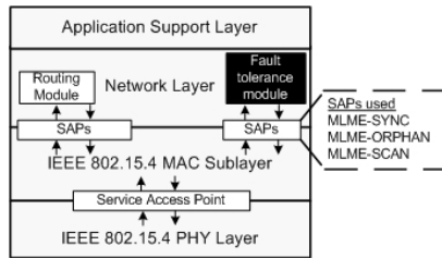
Figure 6. Implementation software architecture
