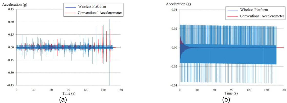
Figure 5 - Time series collected by mote and accelerometer # 03 in the tests of the Pendulum. (a) Response under random excitation in Setup 01 and; (b) Response under ambient noise in Setup 02
