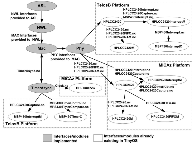
b) TinyOS implementation diagram
