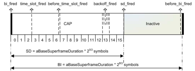
Fig. 6. Asynchronous events
