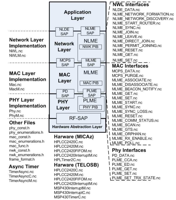
a) Protocol stack architecture
