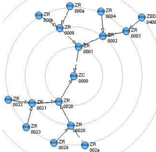
Fig. 10. Experimental network configuration
