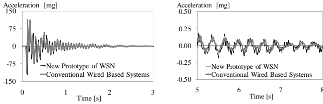
Fig. 9. Time domain series recorded using the developed prototype of WSN platform: (a) High amplitude excitation recordings; and (b) lower amplitude excitation recordings
