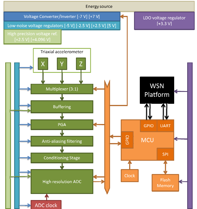
Fig. 5. Sensor Acquisition Board (SAB) architecture
